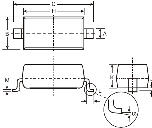
SOD123
