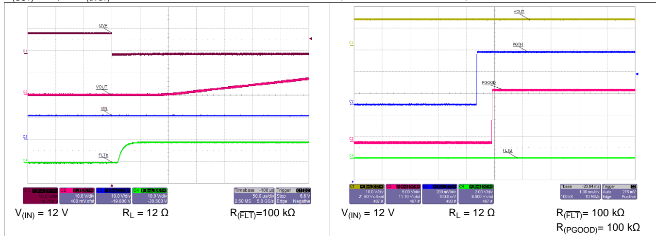
Figure 37. OVP Turn ON delay: OVP \downarrow to Output Ramp \uparrow
