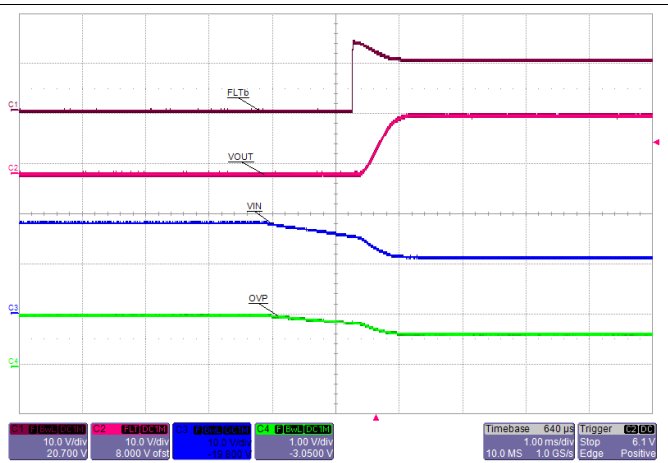
Figure 61. OVP Recovery
