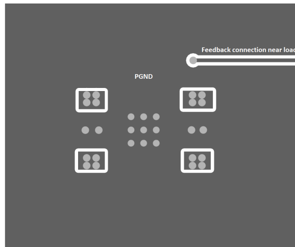
Figure 44. Typical PGND Layer
