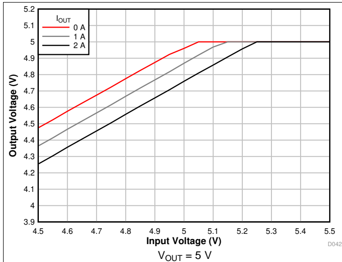
Figure 31. Voltage Dropout
