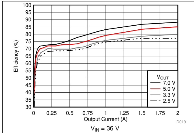
Figure 17. Efficiency versus Output Current
