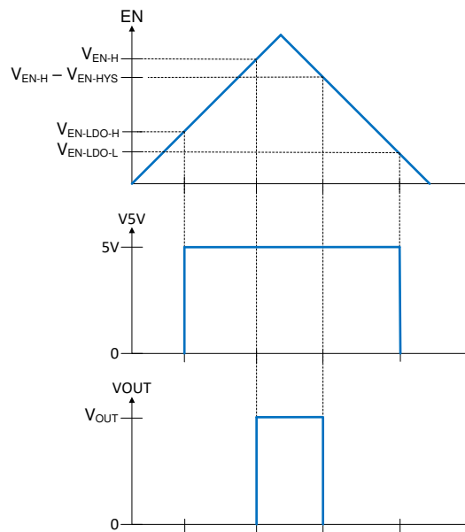
Figure 24. Precision Enable Behavior
