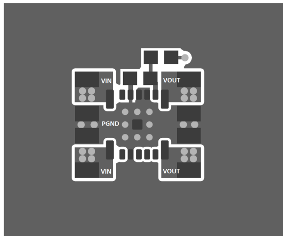
Figure 42. Typical Top-Layer Layout
