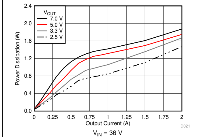
Figure 19. Power Dissipation versus Output Current
