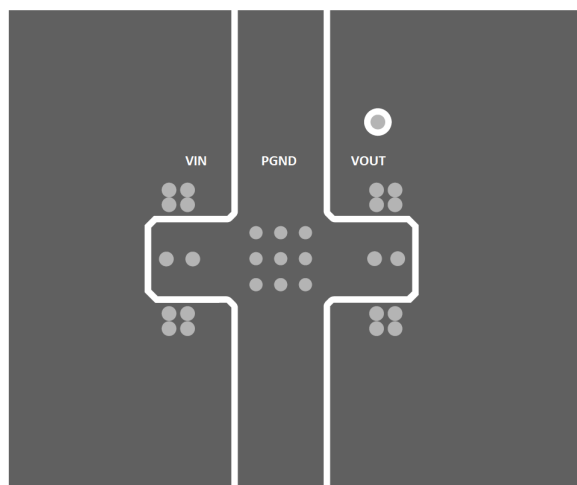
Figure 43. Typical Layer-2 Layout
