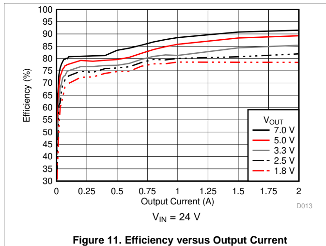
Figure 11. Efficiency versus Output Current
