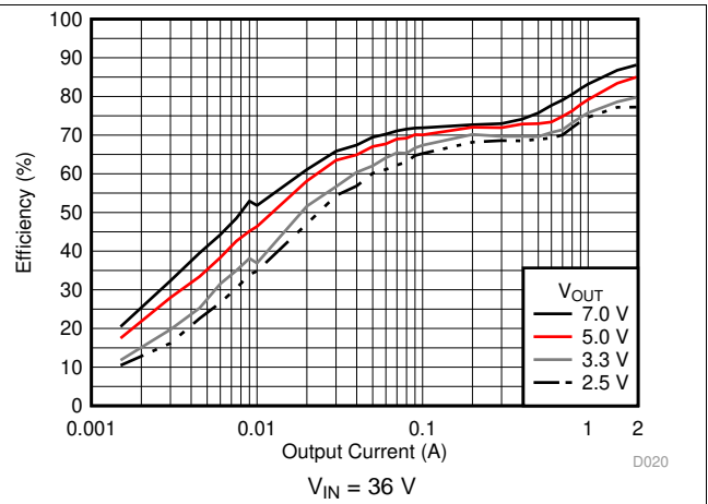
Figure 18. Efficiency versus Output Current
