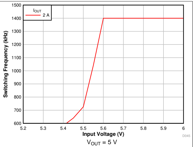
Figure 32. Frequency Foldback
