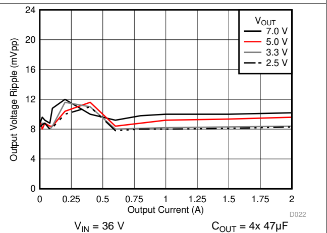
Figure 20. Voltage Ripple versus Output Current
