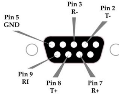
Figure B-21. Pins used on the female RS-232 (DB-9) Serial Connector
