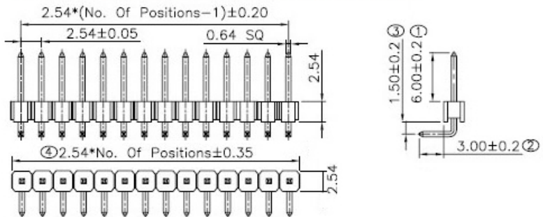
[ 2.00mm Pin Header, Single Row, Right Angle Type, 1*40 Poles ]
