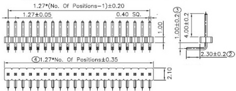
[ 1.27mm Pin Header, Single Row, Right Angle Type, 1*40 Poles ]
