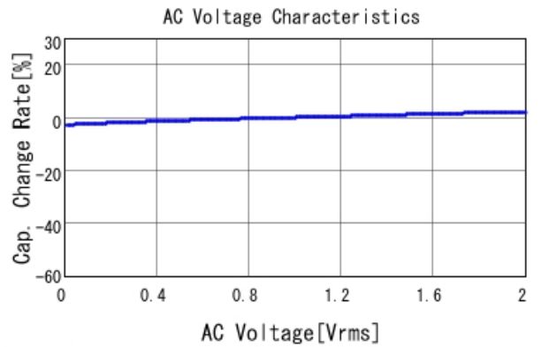
GRM31CR72A105KA01 C-AC Voltage capchange, DCOV, 25
