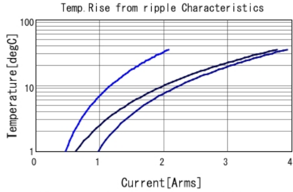
GRM31CR72A105KA01 Temp. rise — 100kHz — 500
