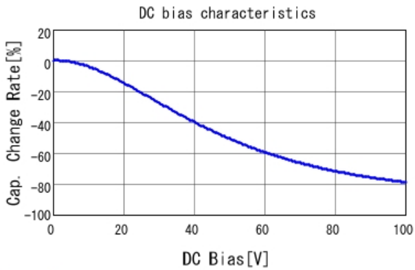
GRM31CR72A105KA01 C-DC bias capchange, 25.0degC, A
