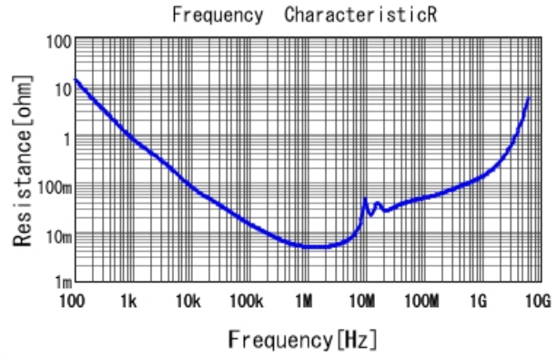
GRM31CR72A105KA01 R DCOV, 25degC
