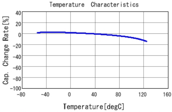
GRM31CR72A105KA01 C-Temp. capchange, DC0.0V, AC1.C
