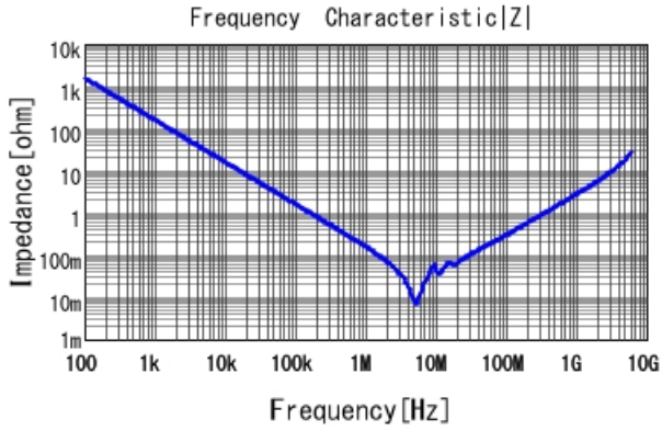
GRM31CR72A105KA01 |Z| DCOV, 25degC
