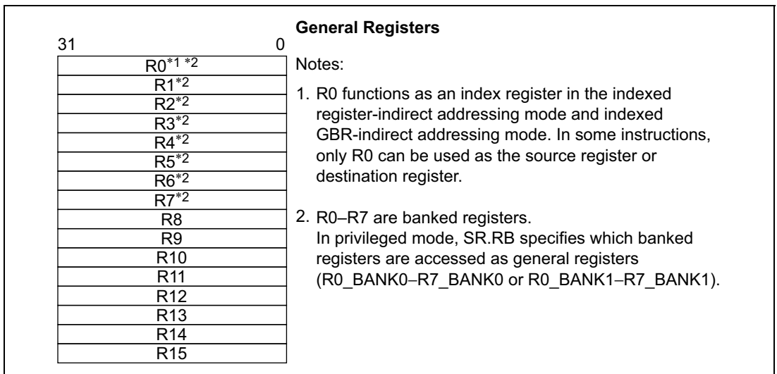
Figure 2.3 General Registers
