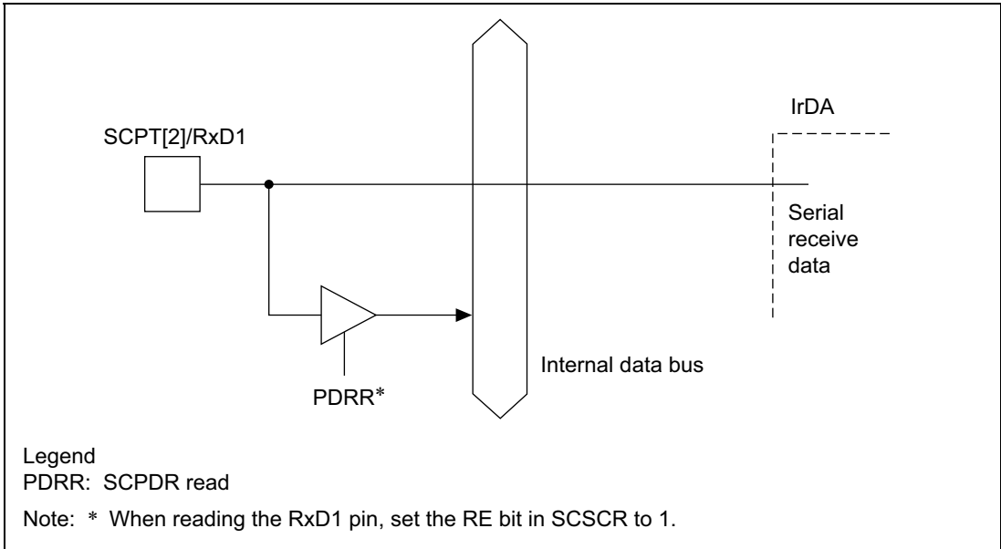
Figure 17.4 SCPT[2]/RxD1 Pin
