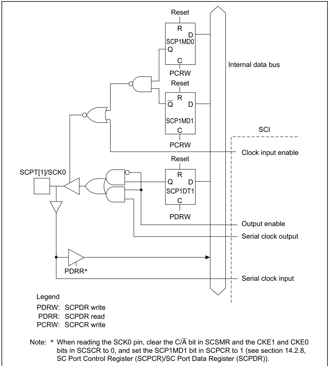
Figure 14.2 SCPT[1]/SCK0 Pin
