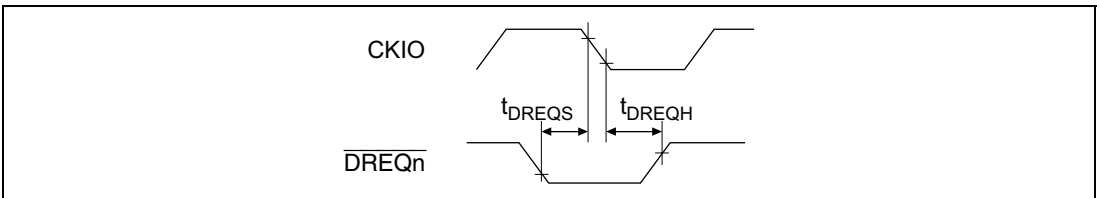
Figure 23.53 \overline{DREQ} Input Timing
