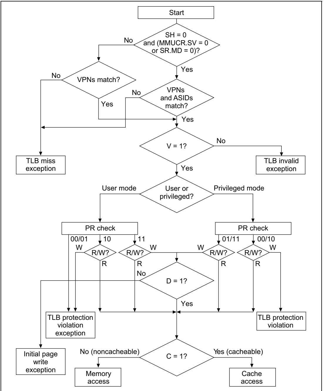
Figure 3.11 MMU Exception Generation Flowchart
