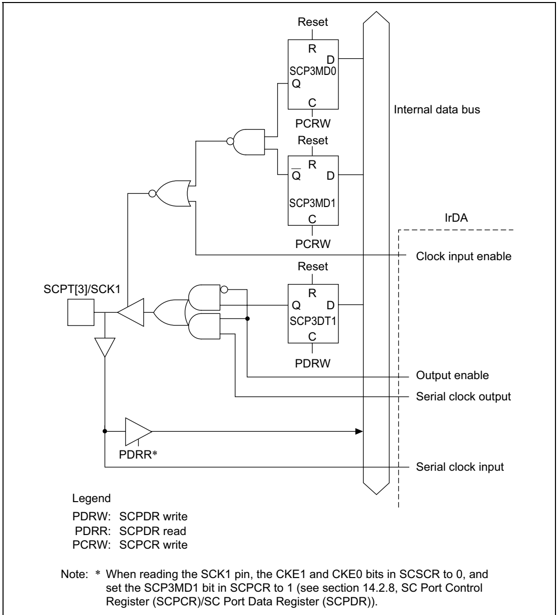
Figure 17.2 SCPT[3]/SCK1 Pin
