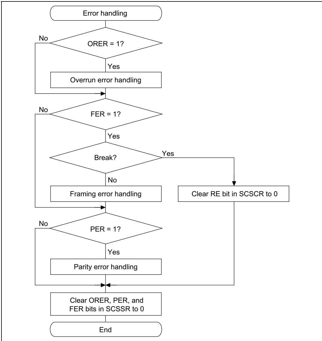
Figure 14.10 Sample Flowchart for Receiving Serial Data (cont)
