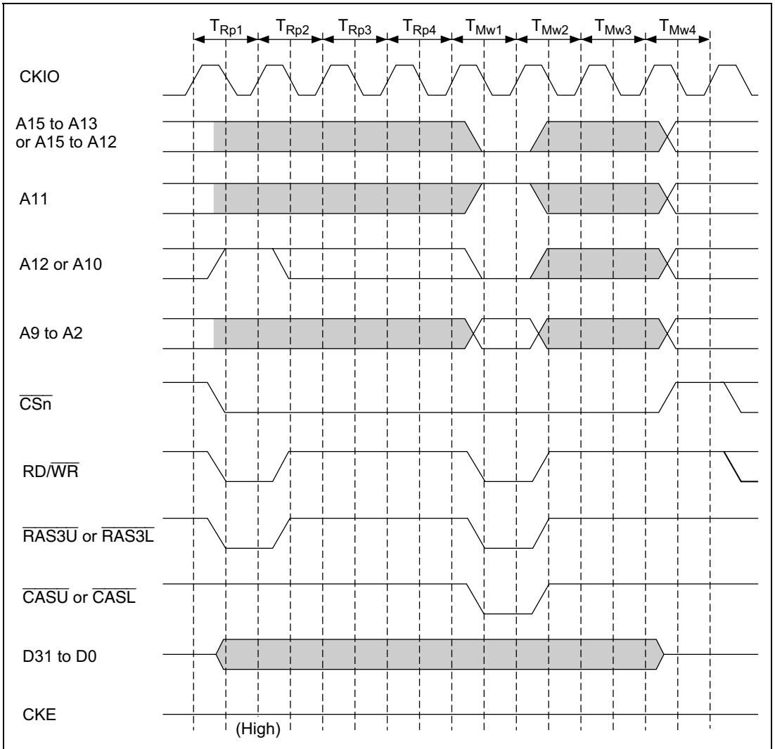
Figure 10.28 Synchronous DRAM Mode Write Timing
