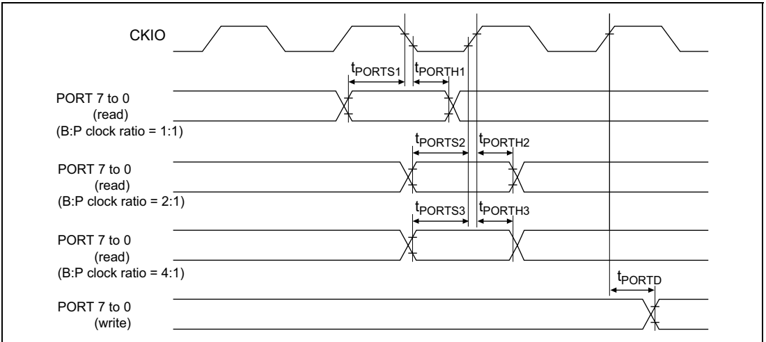
Figure 23.52 I/O Port Timing
