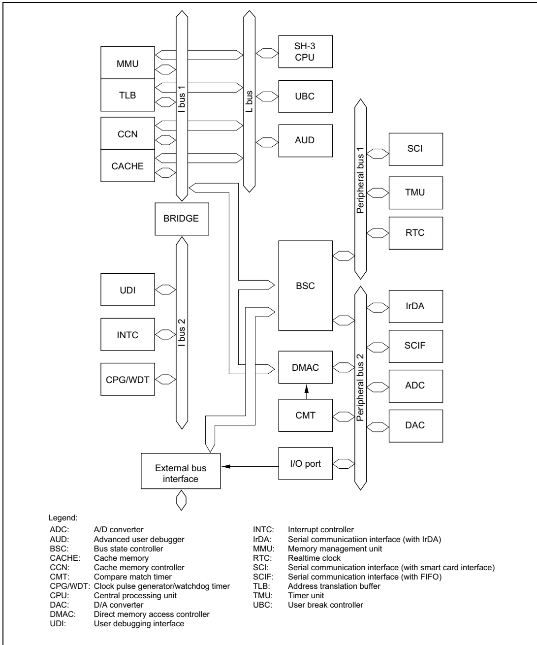
Figure 1.1 Block Diagram
