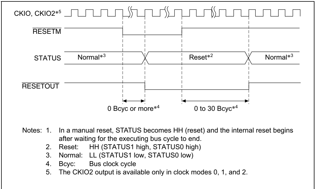
Figure 8.3 Manual Reset STATUS Output
