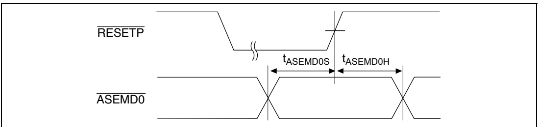
Figure 23.58 \overline{\text{ASEMDO}} Input Timing
