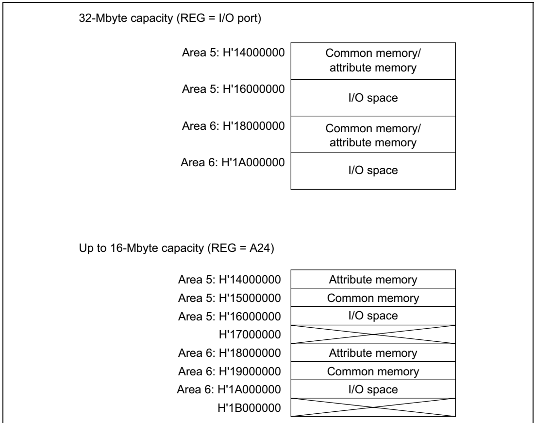
Figure 10.36 PCMCIA Space Allocation
