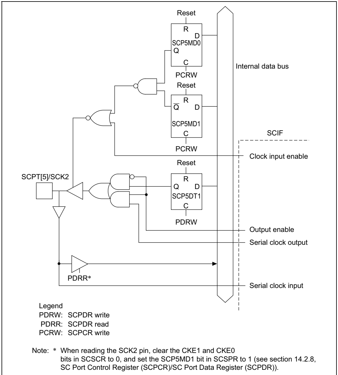
Figure 16.2 SCPT[5]/SCK2 Pin
