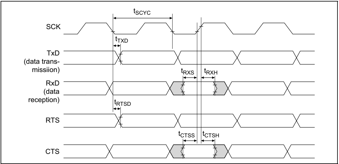
Figure 23.51 SCI I/O Timing in Clock Synchronous Mode
