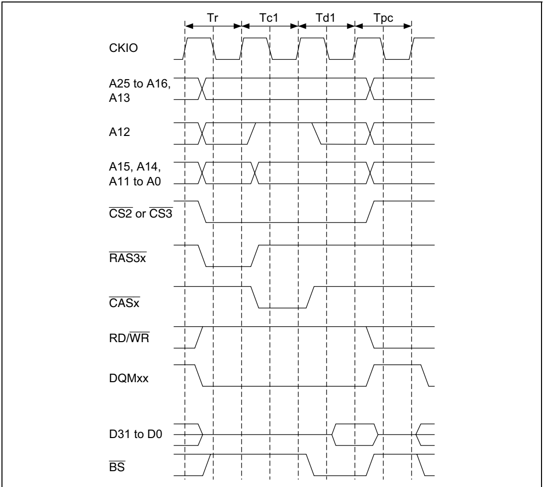
Figure 10.16 Basic Timing for Synchronous DRAM Single Read
