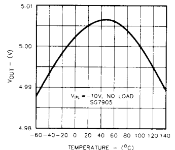
FIGURE 3. TEMPERATURE COEFFICIENT
