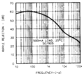
FIGURE 8. RIPPLE REJECTION VS. FREQUENCY
