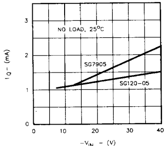
FIGURE 5. QUIESCENT CURRENT VS. V_{IN}
