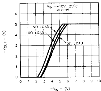
FIGURE 7. DROPOUT CHARACTERISTICS
