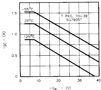
FIGURE 4. SHORTCIRCUIT CURRENT VS. V_{IN}
