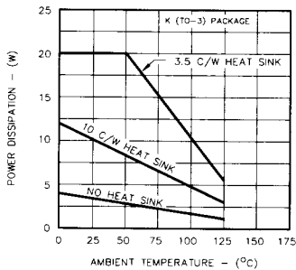
FIGURE 1. MAXIMUM AVERAGE POWER DISSIPATION
