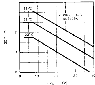
FIGURE 6. SHORT CIRCUIT CURRENT VS. V_{IN}
