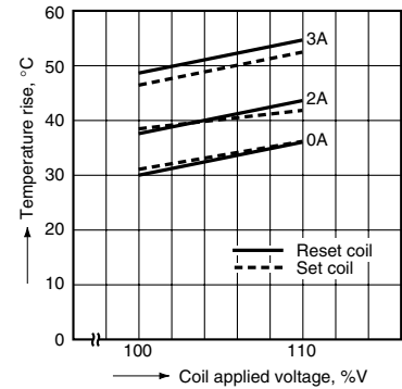
6-(1). Influence of adjacent mounting (1 Form C)
