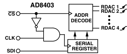
Figure 5. Equivalent Input Control Logic
