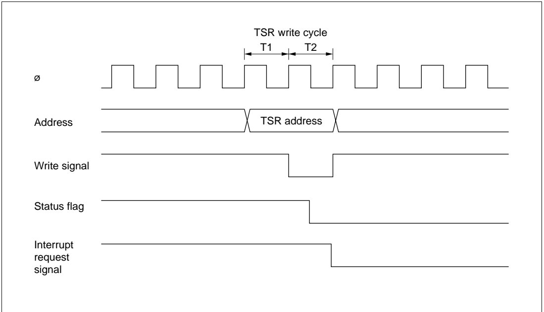
Figure 10-46 Timing for Status Flag Clearing by CPU
