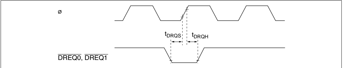
Figure 22-85 DMAC \overline{\text{DREQ}} Input Timing
