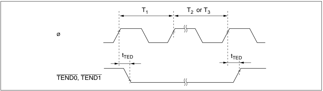
Figure 22-84 DMAC \overline{\text{TEND}} Output Timing
