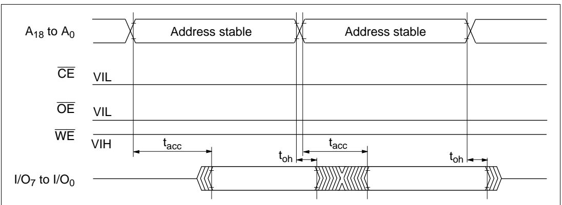
Figure 19-57 Timing Waveforms for \overline{CE}/\overline{OE} Enable State Read
