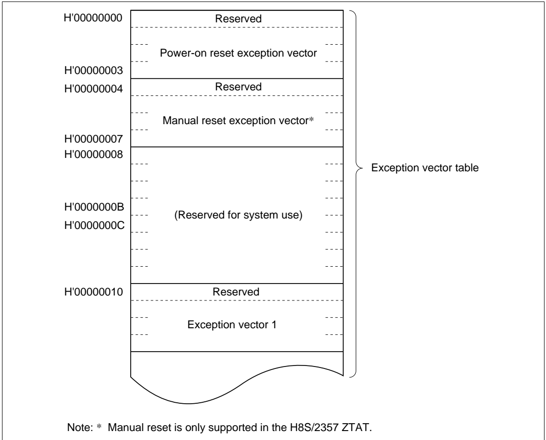
Figure 2-1 Exception Vector Table (Advanced Mode)
