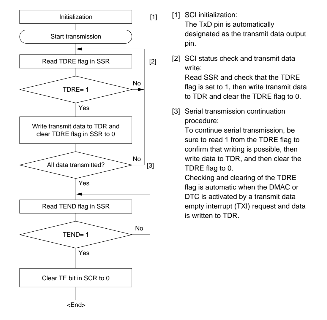
Figure 14-16 Sample Serial Transmission Flowchart
