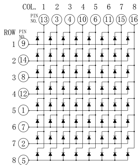
Common Row Anode: KWM-30881AVB
