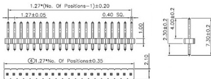
[ 1.27mm Single Row Pin Header , Straight Type , 1*40 Poles ]
