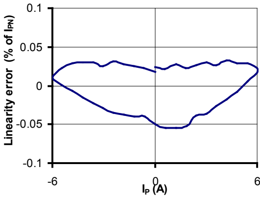
Figure 1: Linearity error
