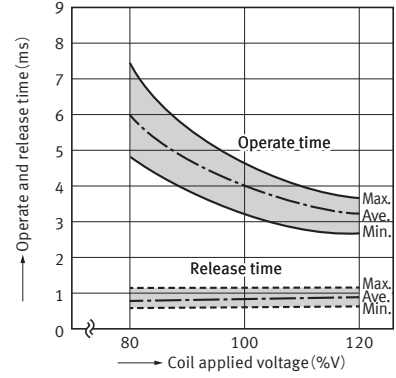
4.-(6) Operate & release time (with diode, 2 Form A)
