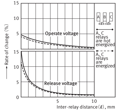
6.-(3) Influence of adjacent mounting (2 Form A)
