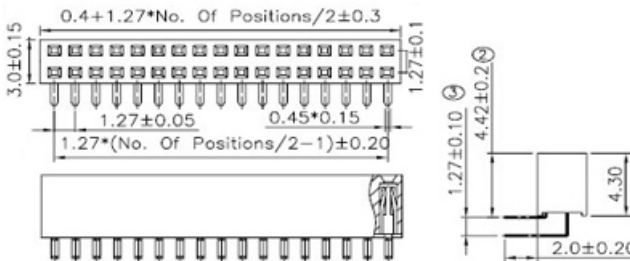
[ 1.27mm Female Header, 2 Rows, Right Angle Type , 2*40 Poles ]
