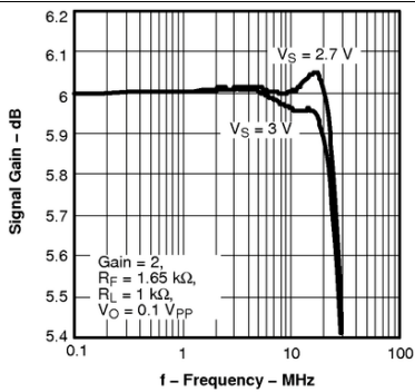
Figure 13. Frequency Response
