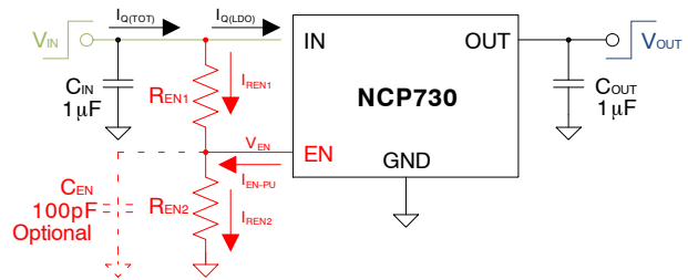
Figure 74. Circuit – IN Voltage UVLO by EN Pin
